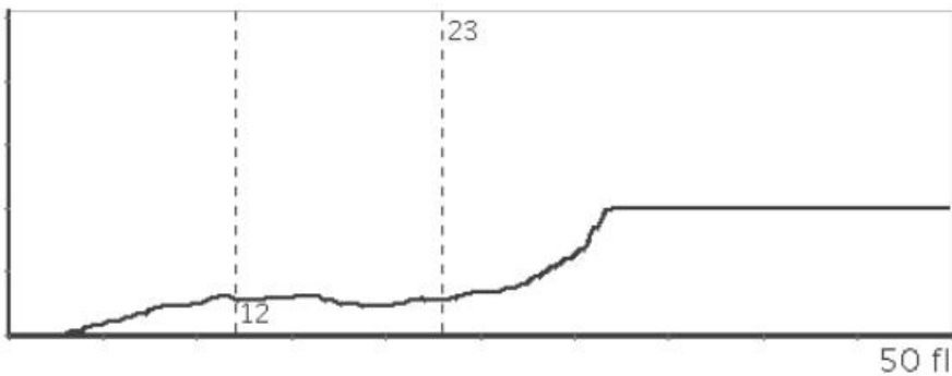
RBC Histogram
